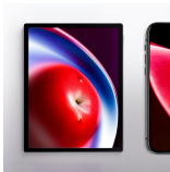
step 1000
